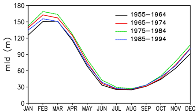
Figure 9. Seasonal changes of mixed layer depth averaged over the North Pacific (150°E~140°W, 30°N~50°N) in 1955–1964 (black solid line), 1965–1974 (red solid line), 1975–1984 (green dashed line), and 1985–1994 (blue dashed line).
